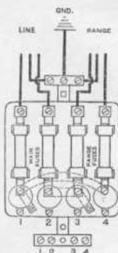
Wiring Diagram of No. 264, ER264, 464 and Similar
