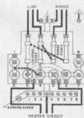
Wiring Diagram of Nos. 268C, 468C and Similar
